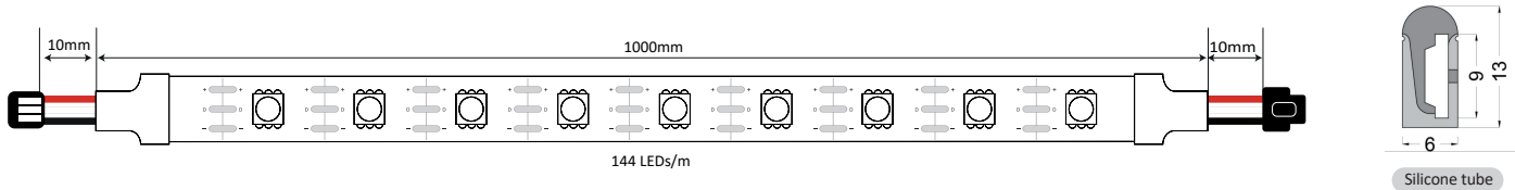
RGBW 144 LEDs(1 meter single length Mechanical Diagram
