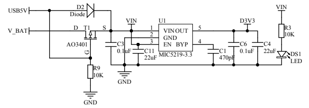
Charger and Li-Battery(1-cell)
