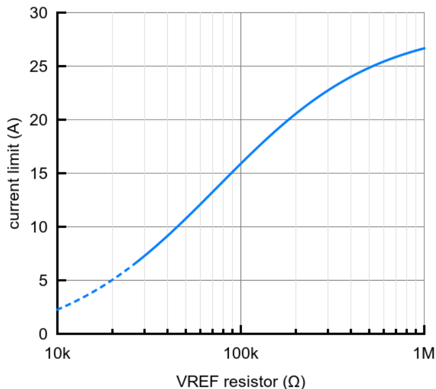
Pololu G2 High-Power Motor Driver 24v13 current limit vs. VREF resistor
