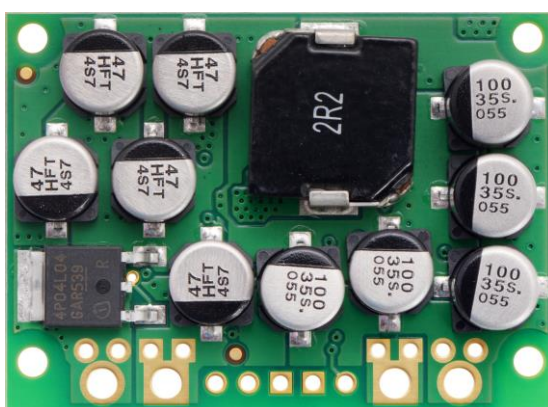
Pololu 7,5V, 15A Step-Down Voltage Regulator D24V150F7, top view.
