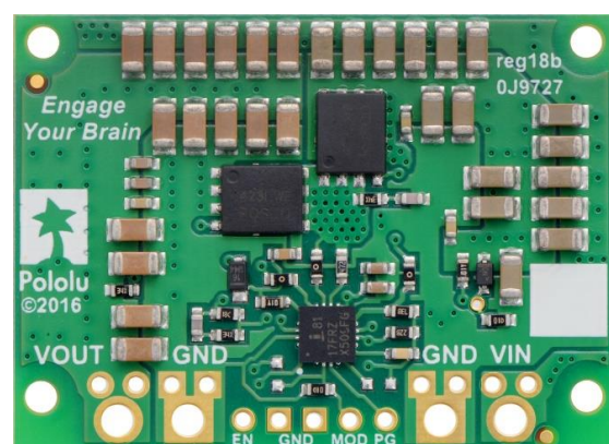
Pololu 7,5V, 15A Step-Down Voltage Regulator D24V150F7, bottom view.
