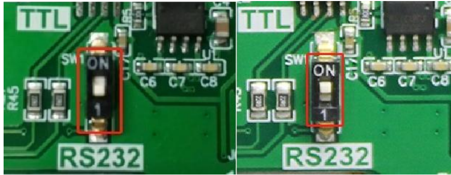
Diagram 7-1 RS232/TTL level
