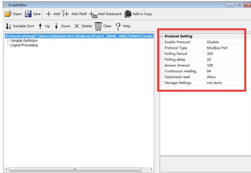
Diagram 8-2 Protocol configuration
