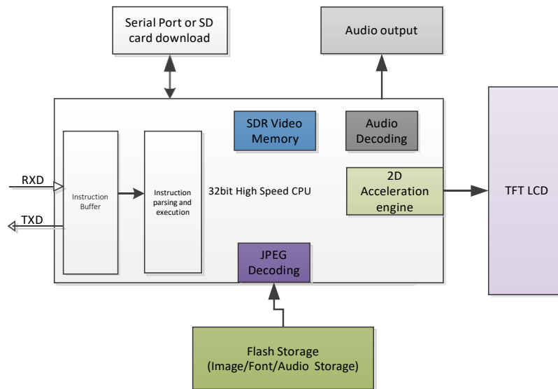
Diagram 11-1 M series product internal structure diagram of serial screen
